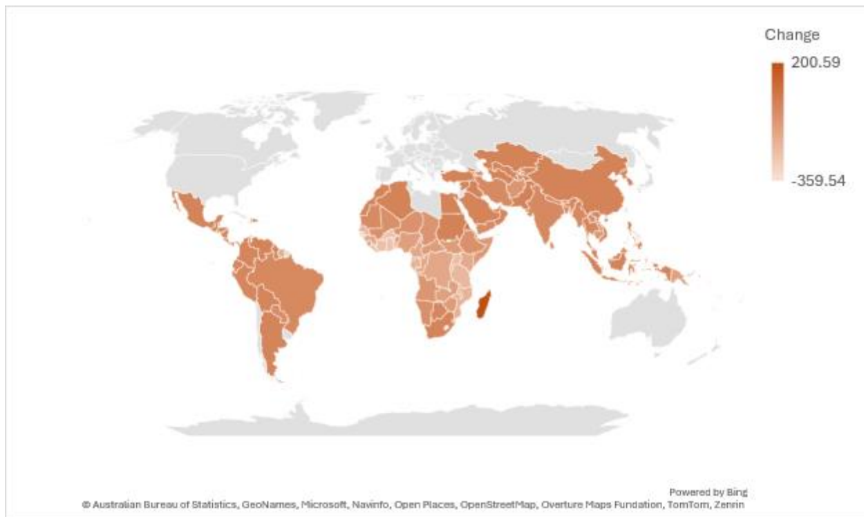
Figure 1: Change in malaria incidence rate across 103 countries between 2000 and 2024.
